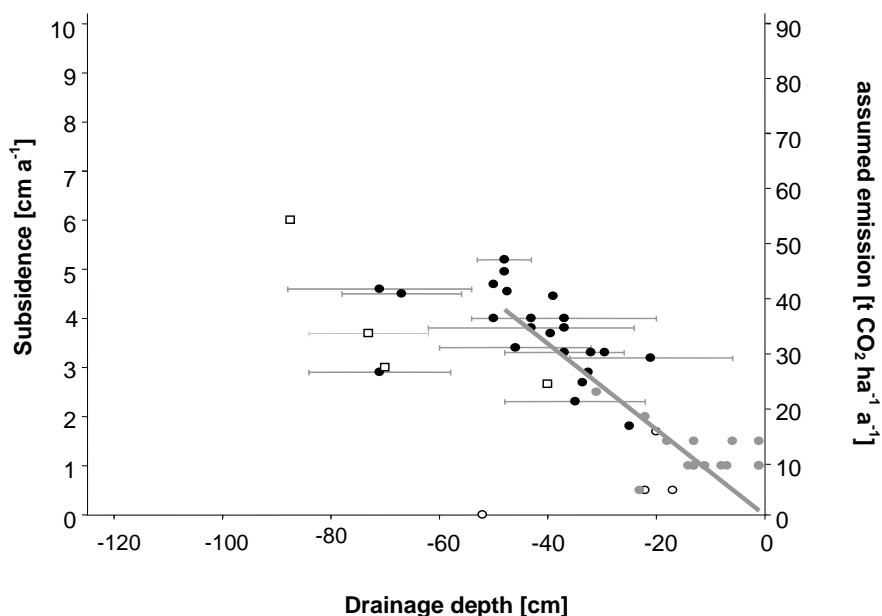
Figure 2.4.3. Relation between drainage depth and CO 2 emissions from peat decomposition in tropical peat swamps 41 . Rate of subsidence in relation to mean annual water level below surface Horizontal bars indicate standard deviation in water table (where available). Open circles denote unused, drained forested sites. Land use: (□) agriculture, (●) oil palm (recorded 13 to 16 or 18 to 21 years after drainage), (●) degraded open land in the Ex Mega Rice Project area, recorded ~10 to ~12 years after drainage, (○) drained forested plots, recorded ~10 to 12 years after drainage. The slope of the line represents 0.9 t CO 2 /ha emitted per 1 cm drained.
