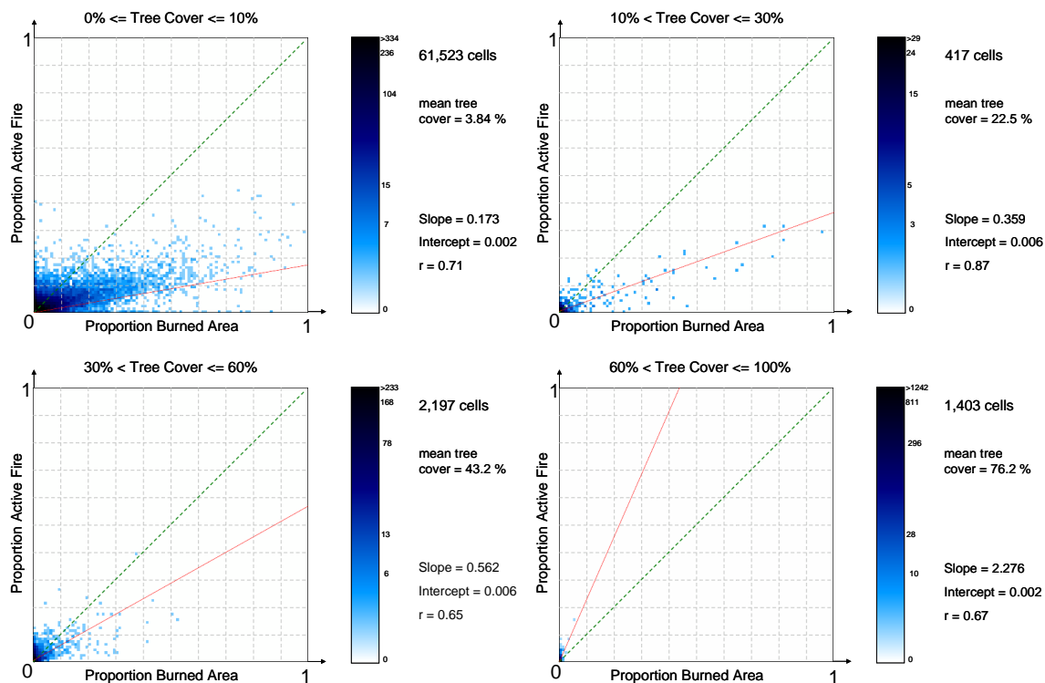
Figure 2.6.2. Scatter plots of the monthly proportions of 40x40km cells labeled as burned by the 1km active fire detections plotted against the proportion labeled as burned by the 500m burned area product, for four tree cover class ranges, globally, period July 2001 to June 2002. Only cells with at least 90% of their area meeting these tree cover range criteria and containing some proportion burned in either the active fire or the monthly burned area products are plotted. The Theil-Sen regression line is plotted in red; the white-blue logarithmic color scale illustrates the frequency of cells having the same specific x and y axis proportion values (Source: Roy et al, 2008).
