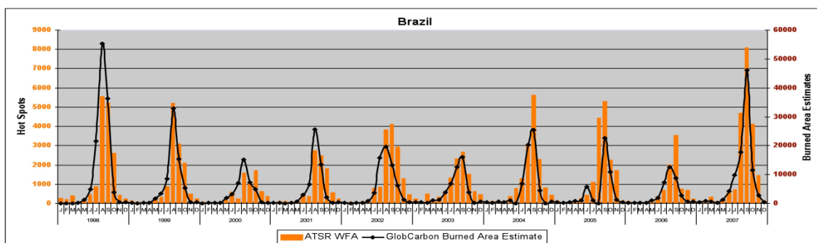
Figure 2.6.1. Temporal comparison between ATSR World Fire Atlas nighttime active fire counts and Globcarbon 59 burned area estimate in km 2 . While the two products display the same temporal pattern, the areal extent is different by almost an order of magnitude, highlighting the under-sampling issues of active fire products.
